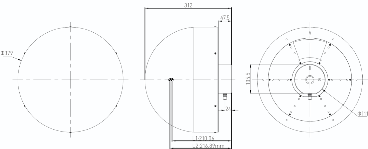
Top view Bottom View
